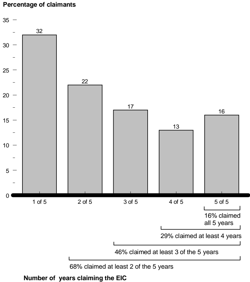
Figure 2: Number of Years the EIC Was Claimed in a 5-Year Period by Taxpayers Who Claimed the EIC for Families With Children at Least Once in Tax Years 1990 Through 1994
