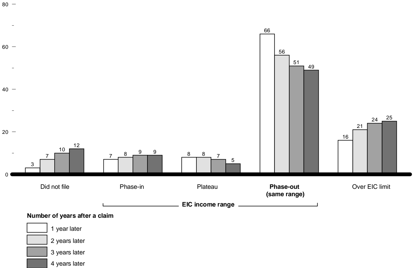
Figure 7: Changes in Income for EIC Claimants Who Claimed the Credit With Reported Income in the Phase-Out Range
