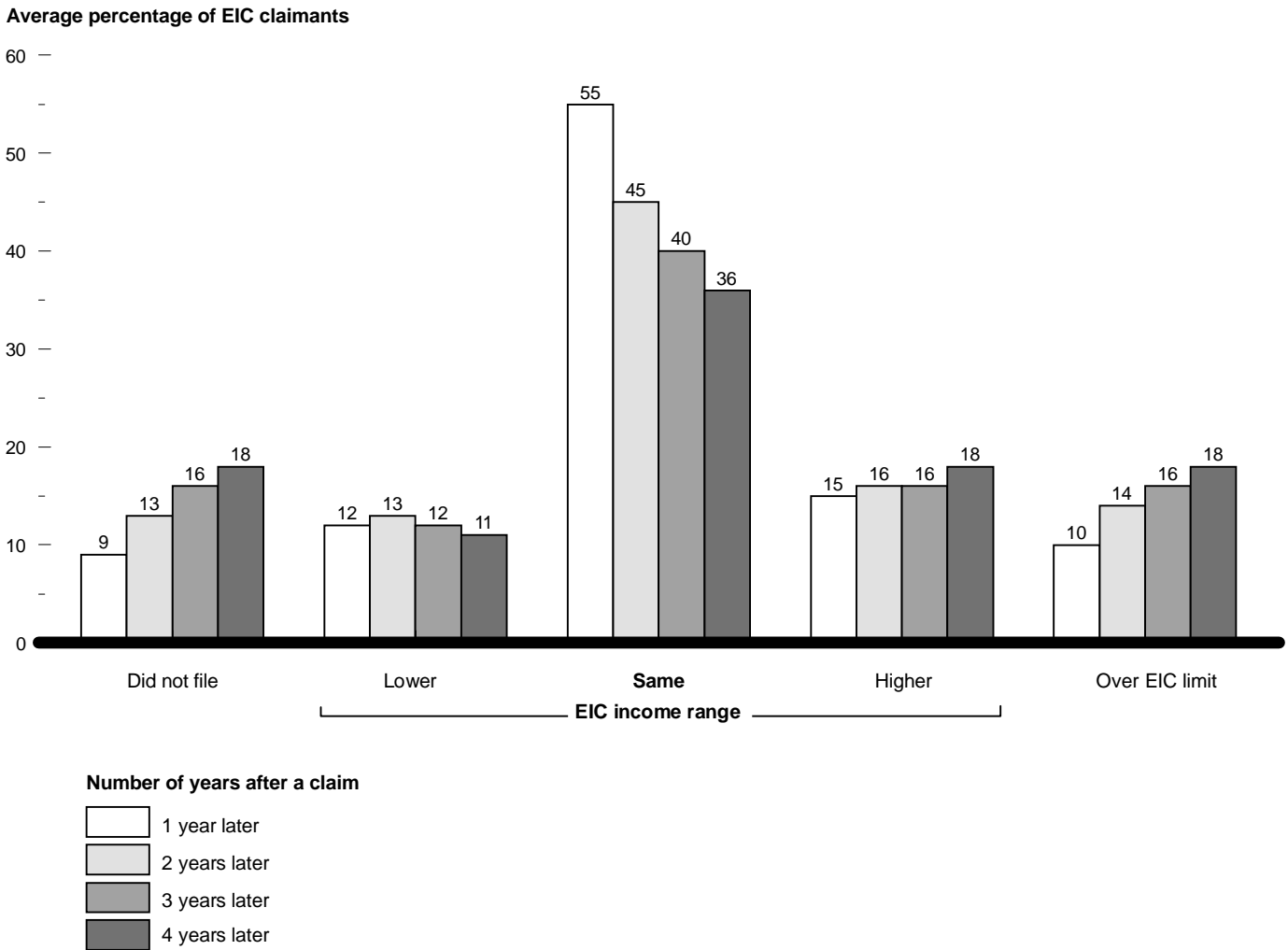
Figure 5: Changes in EIC Claimants' Reported Income Relative to EIC Income Ranges, From 1 to 4 Years After an EIC Claim
